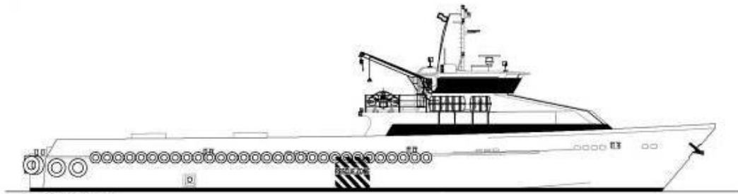
STBD PROFILE SCALE 1:100 AGAVE 500L
