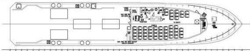
MAIN DECK SCALE 1:200
